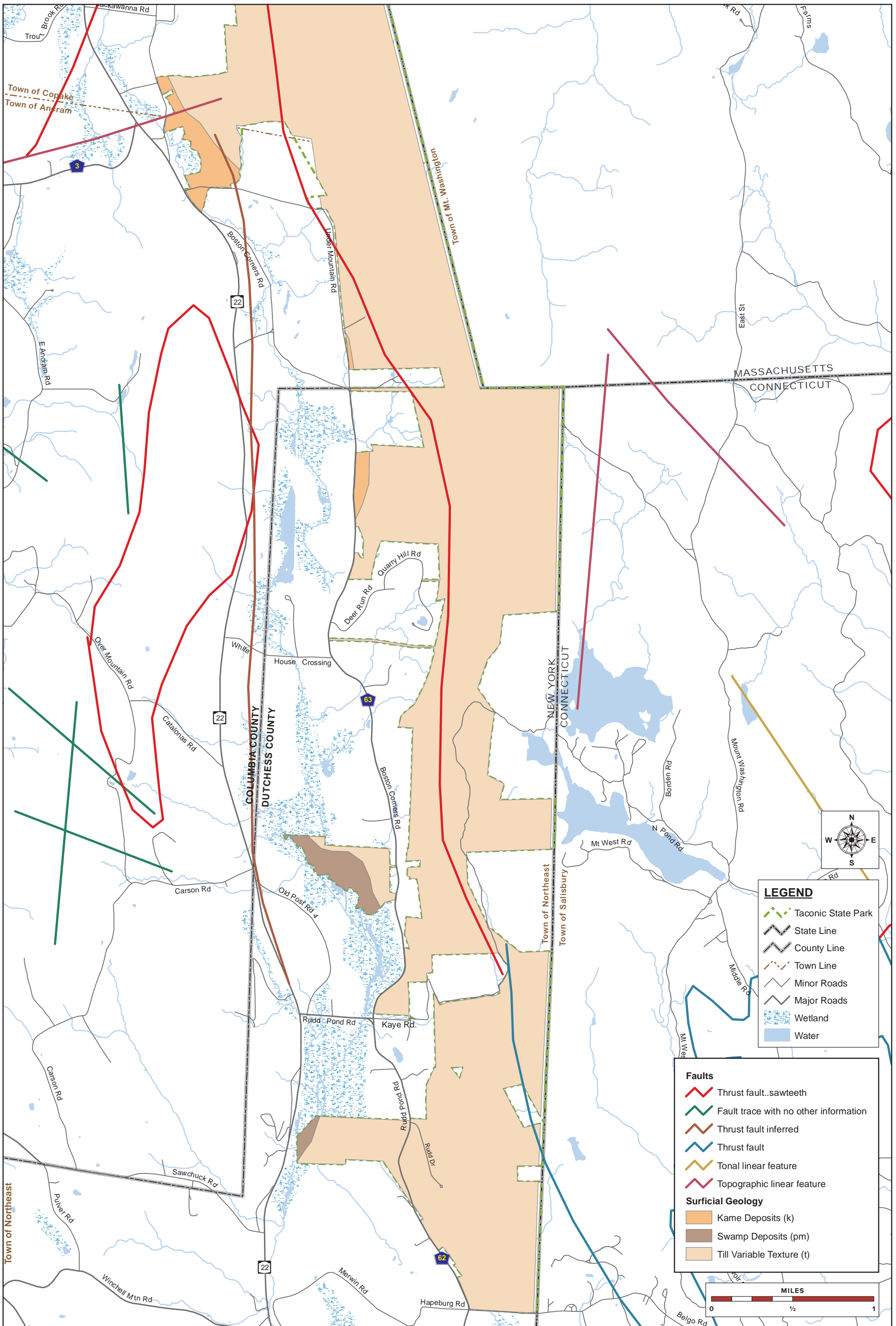
Figure 4B - SURFICIAL GEOLOGY SOUTHERN SECTION
